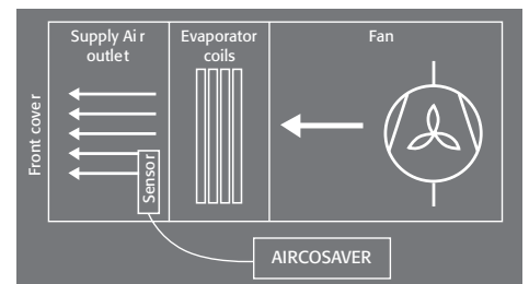
8 Position sensor in supply air stream (schematic)
